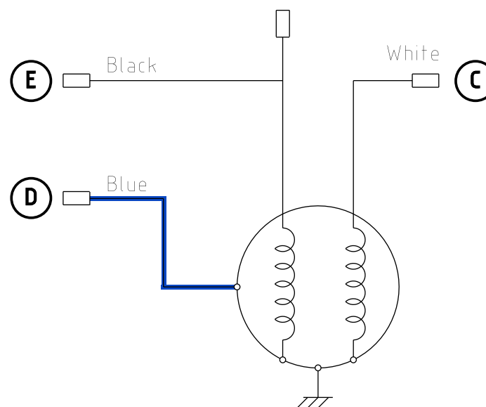
MAGNETO 928.555.002
