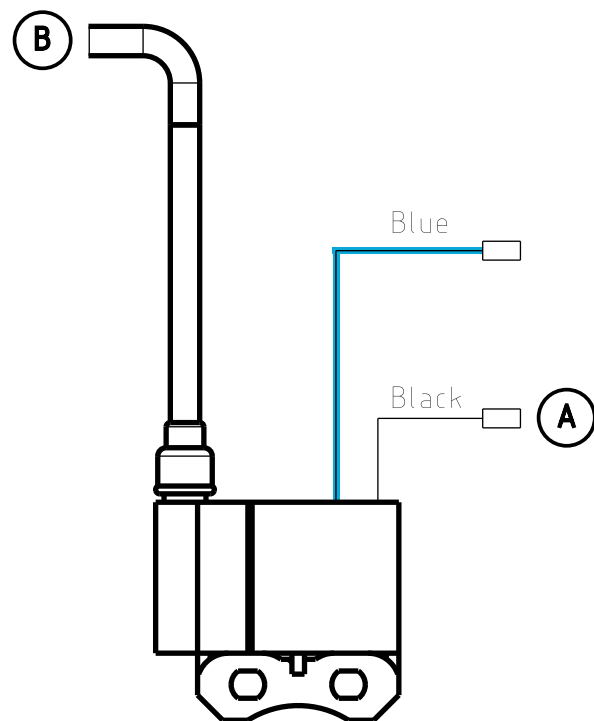
COIL 928.600.001
